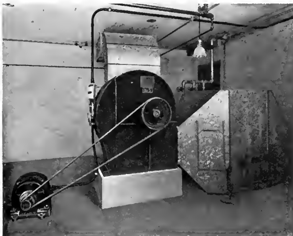
MODEL INSTALLATION IN BASEMENT OF INSTITUTE OF THERMAL RESEARCH, BUFFALO, N. Y.
